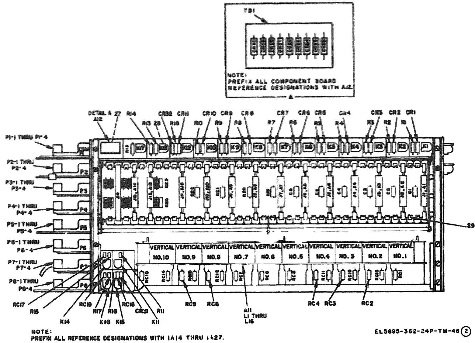
Figure 56. Code Switch Matrix and Amplifier TA-894/GTC (Sheet 2 of 2).
