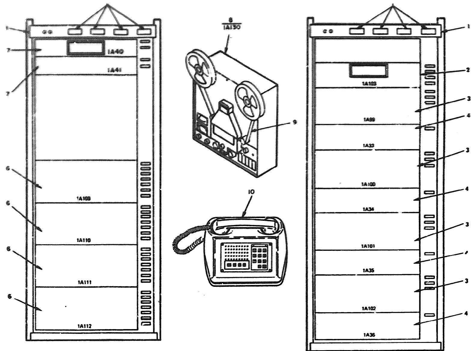
Figure 1. Upright Assembly C-A8253, Front View; Recorder RD-374/U; Upright Assembly C-A8254, Front View; Telephone TA-900/G.
