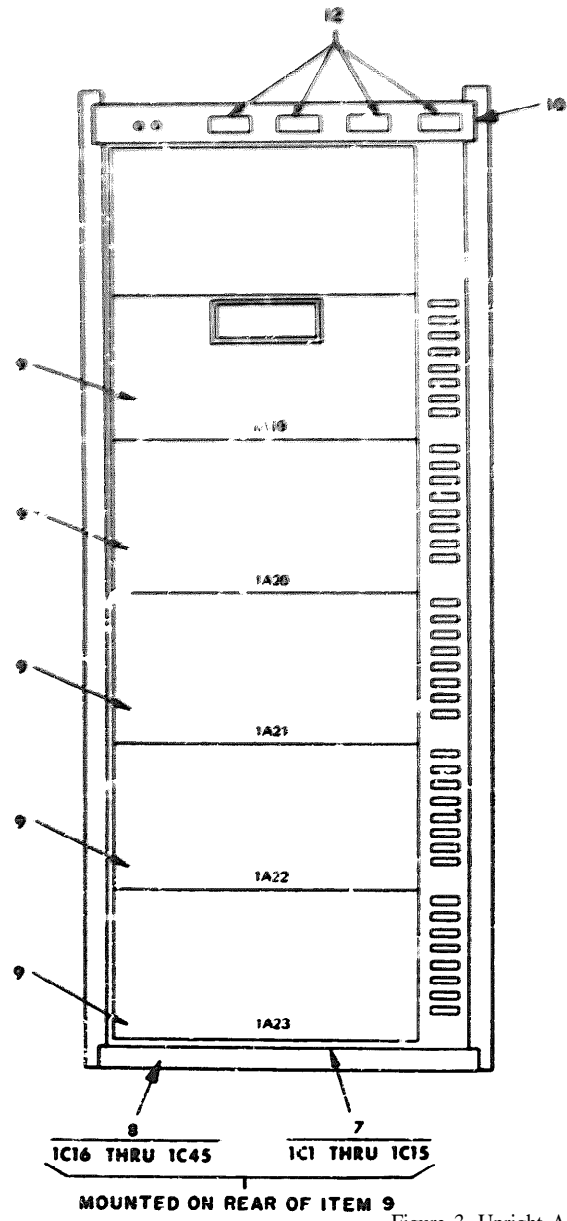
Figure 3. Upright Assembly C-A8257, Front View; Upright Assembly C-A8258, Front View.
