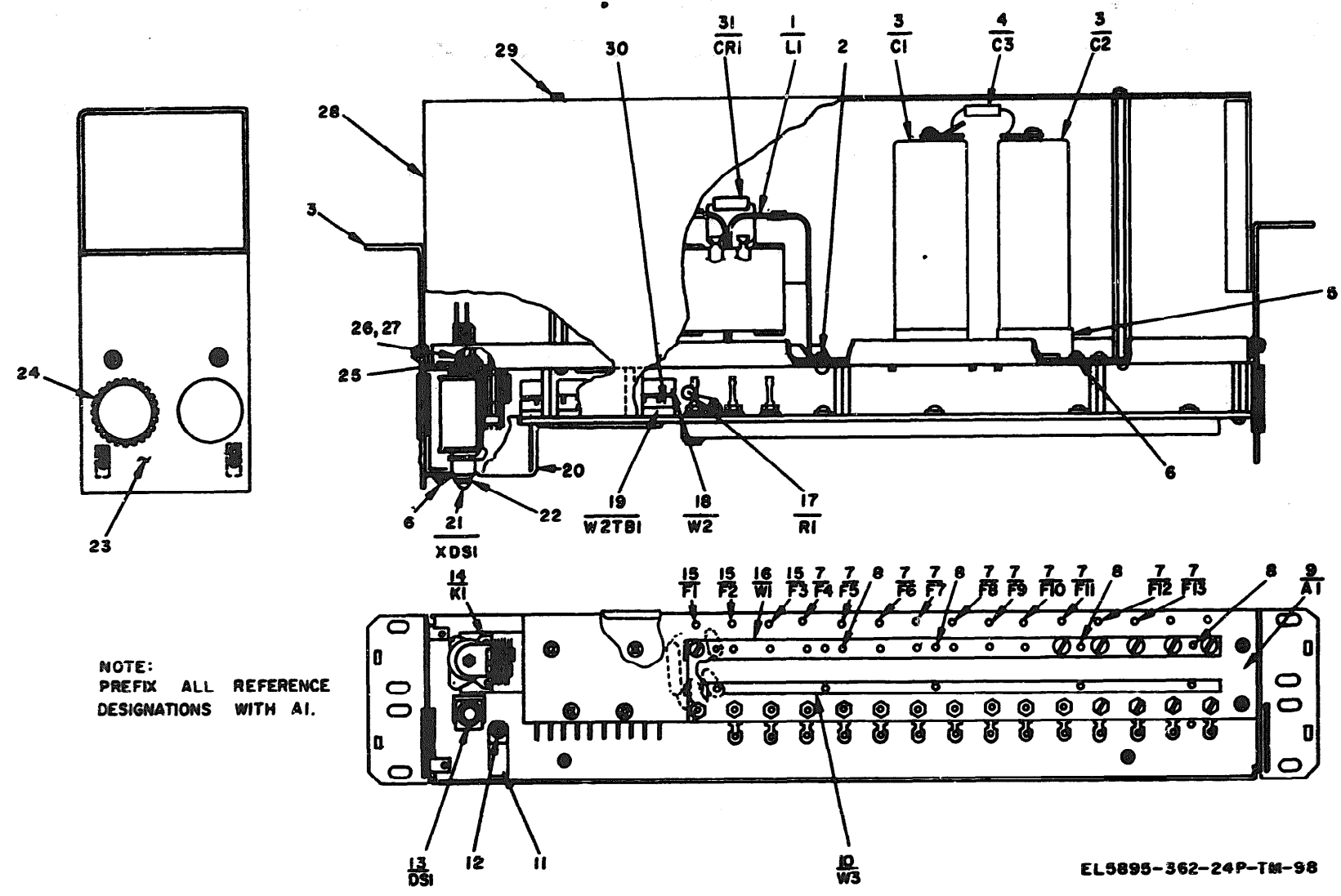
Figure 113. Fuse Panel, Inband Signaling.
