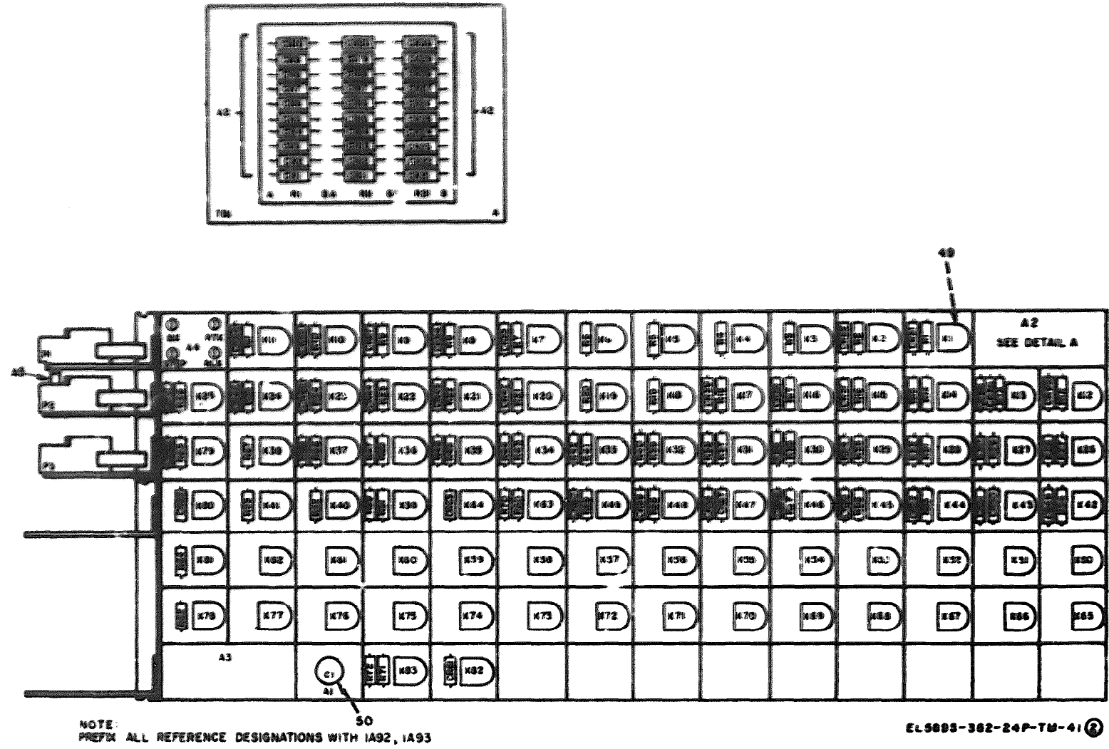
Figure 50. Marker Circuit-B TA-892/GTC (Sheet 2 of 2).
