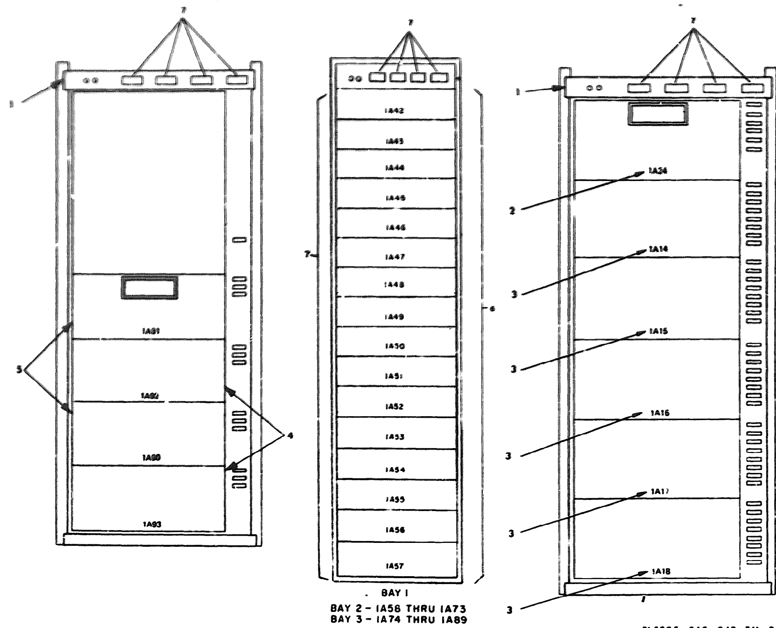
Figure 2. Upright C-A8255, Front View; Upright Assembly C-A8252, Front View; Upright Assembly C-A8256, Front View.
